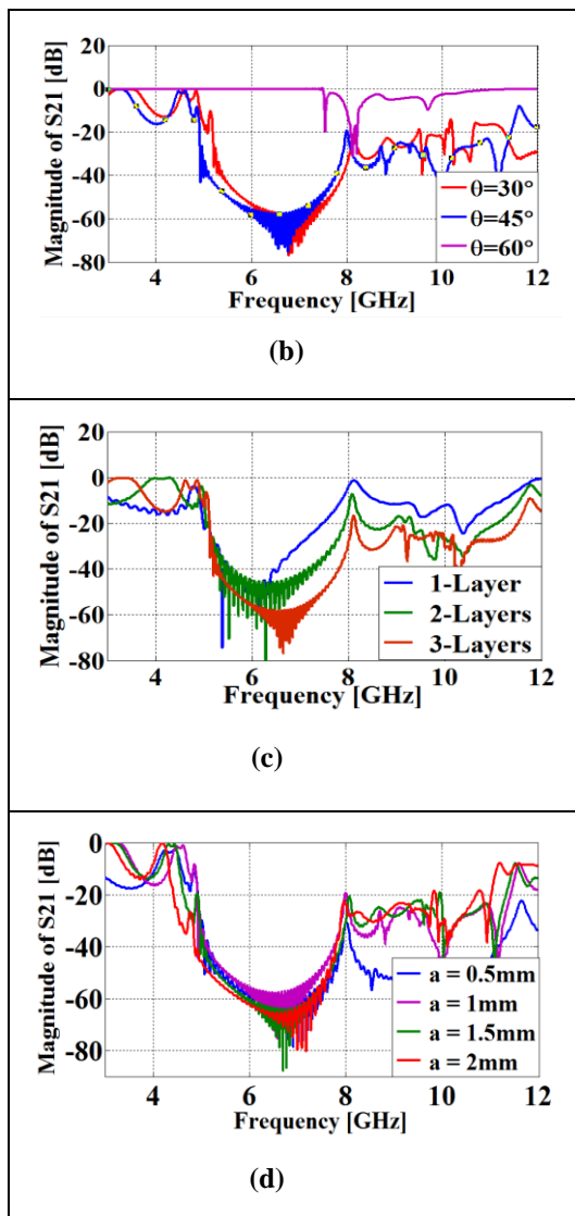
Fig.4. (a) The transmission coefficient S_{21} for different patch sizes 2.8mm, 3mm, 3.2mm, (b) S_{21} for 3-layers EBG structure with different rotations angle \theta , (c) The transmission coefficient S_{21} for EBG structure with \theta of 45^\circ for different number of layers, (d) The transmission coefficient S_{21} of EBG structure with different gap distance between the circular alignment layers.
